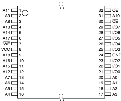
TSOP Top View (8 x 20 mm) Type 1
